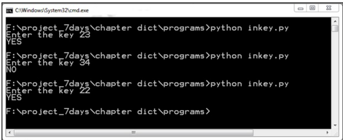
Output of in program
