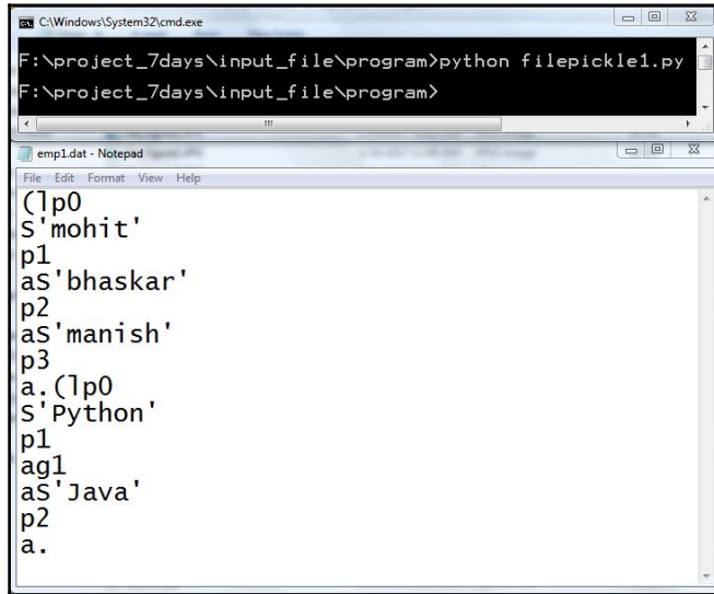
Output of pickle file
