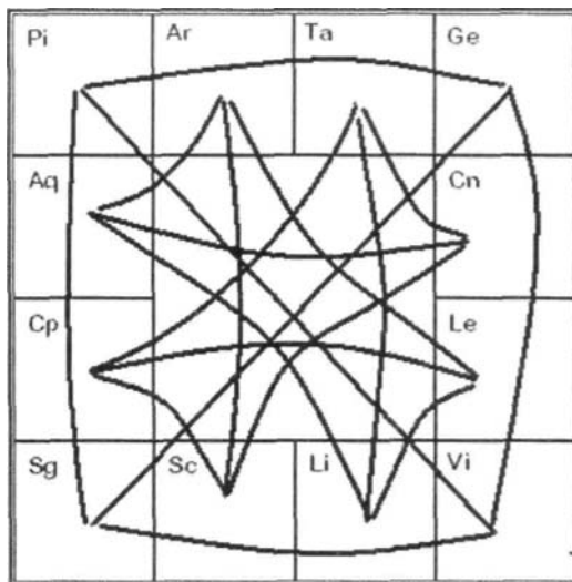
Figure 2: Rasi Aspects
