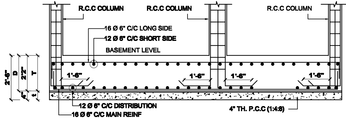
FOOTING -F1 TO F10 SECTION = AA
