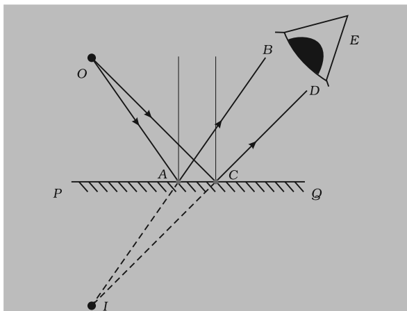
Fig. 16.5 : Image formation in a plane mirror appear to come from the point I. Since the reflected rays do not actually meet at I, but only appear to do so, we say that a virtual image of the point O is formed at I. As you have learnt already in Class VII, such an image cannot be obtained on a screen.
