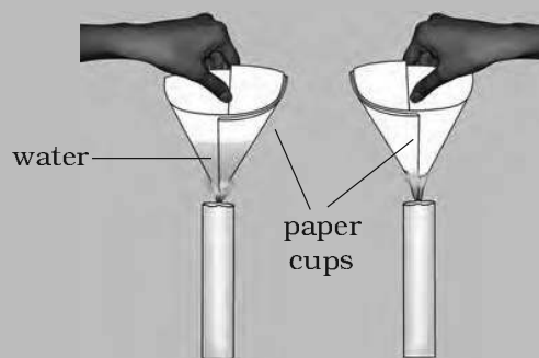
Fig. 6.5 : Heating water in a paper cup
