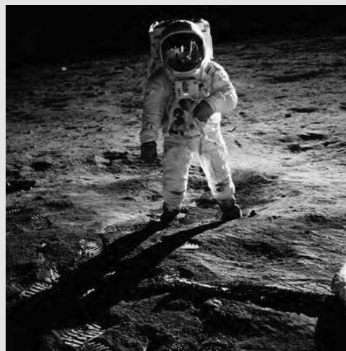
Fig. 17.8 : An astronaut on the moon
