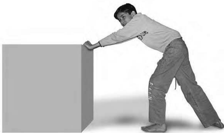
Fig. 12.6 : You have to push on the box to keep it moving
