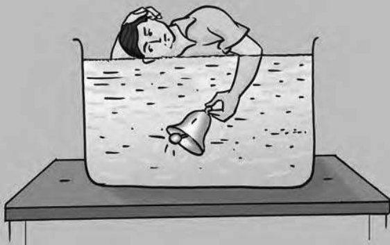
Fig. 13.11 : Sound travelling through water
