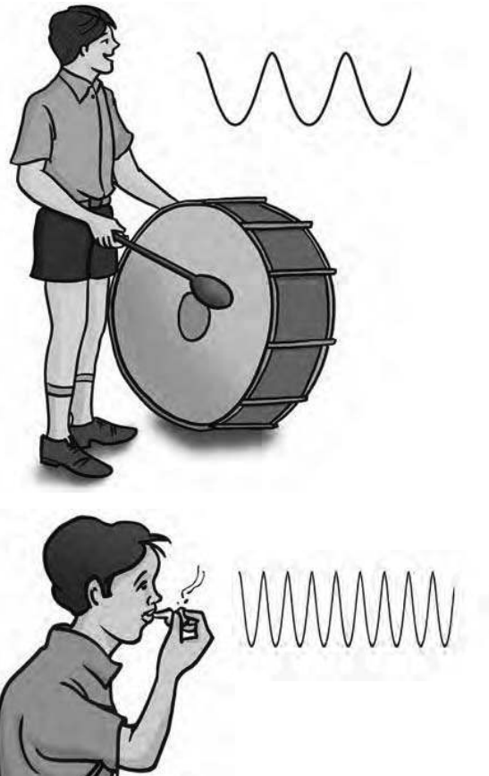
Fig. 13.18: Frequency determines the pitch of a sound
