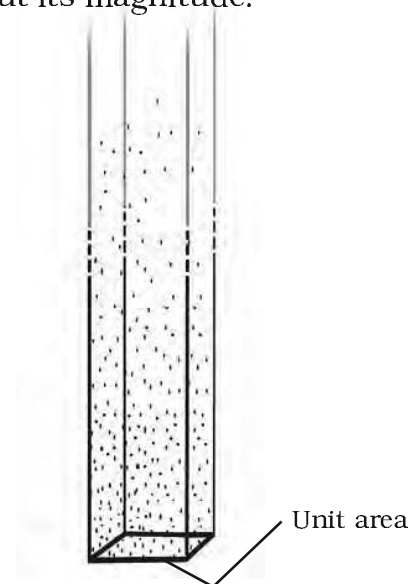
Fig. 11.17 : Atmospheric pressure is the weight of air in a column of unit area
