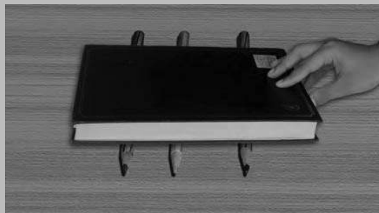
Fig. 12.15 : Motion of the book on rollers
