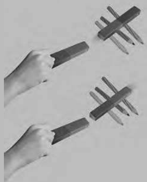
Fig.11.10 : Observing attraction and repulsion between two magnets
