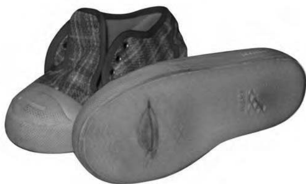
Fig. 12.8 : Soles of shoes wear out due to friction
