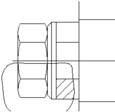
Figure 243. Cutaway Hole and Hidden Lines
