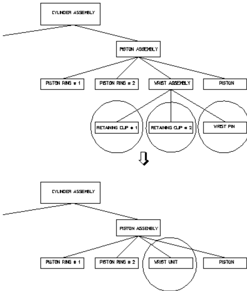
Figure 217. Smashing Parts
