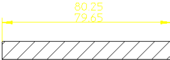
Figure 124. Limit Tolerancing
