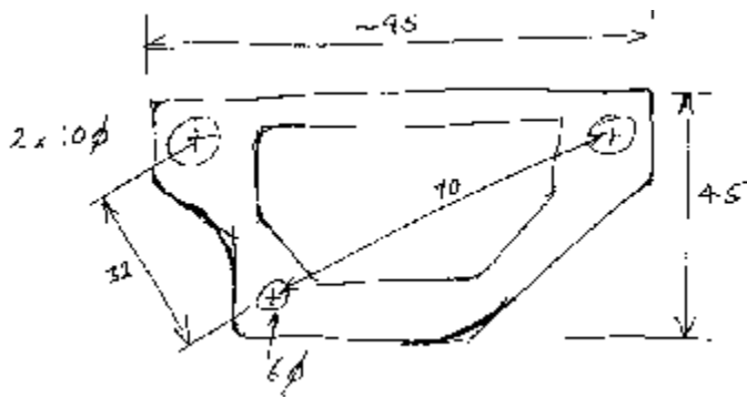
Figure 30. Design Sketch
