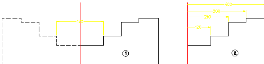
Figure 102. Symmetry-Style Dimensioning
