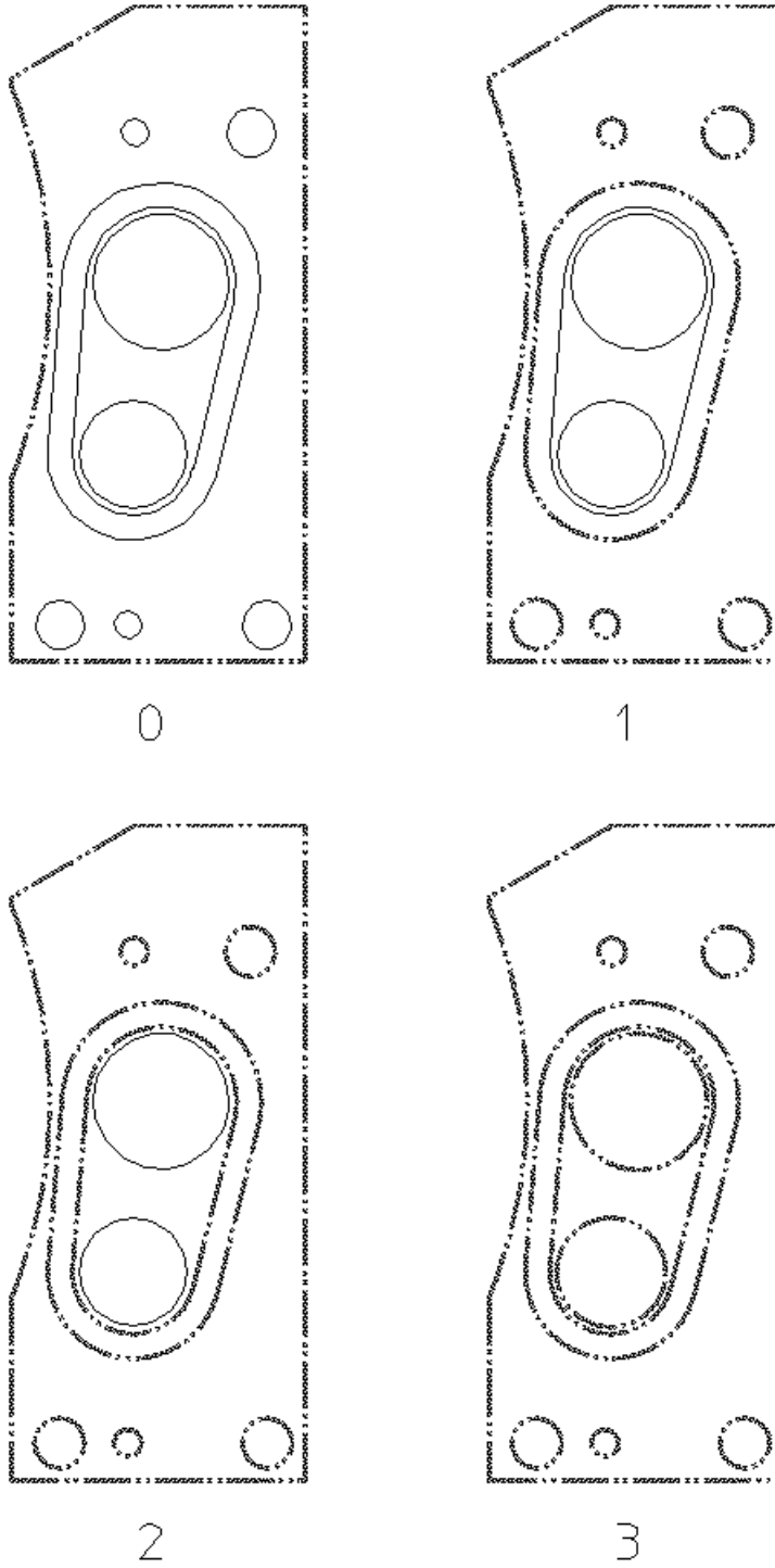
Figure 10. Contour Levels
