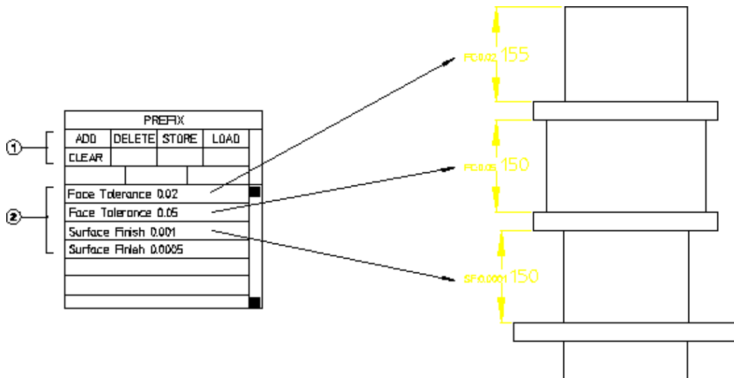
Figure 125. Drawing Prefixes
