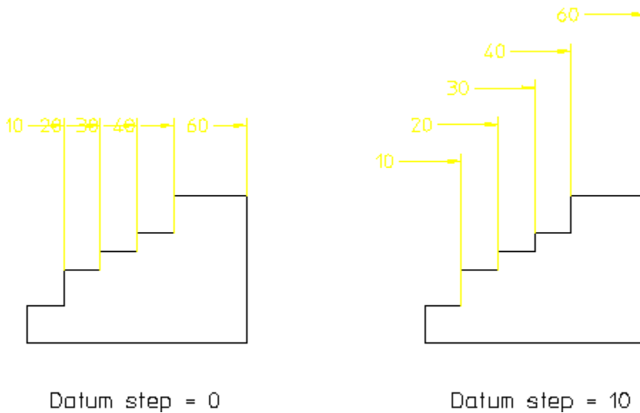
Figure 132. Datum Stepping
