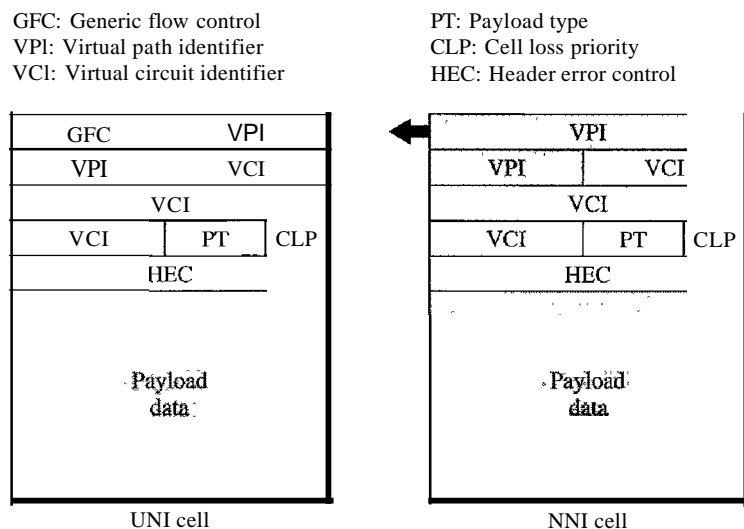
Figure 18.19 ATM headers
